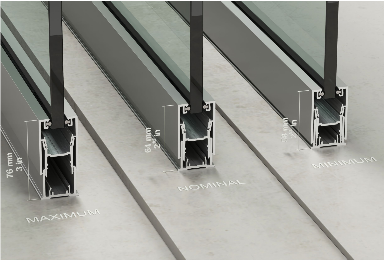
BASE ADJUSTMENT
