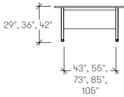
Rec Single Top Workshop Table (ESTMA)
