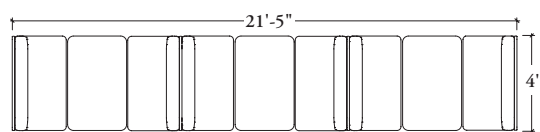
Banqs Single-Sided Sofas, Low Screens, wrapped in architectural walls
