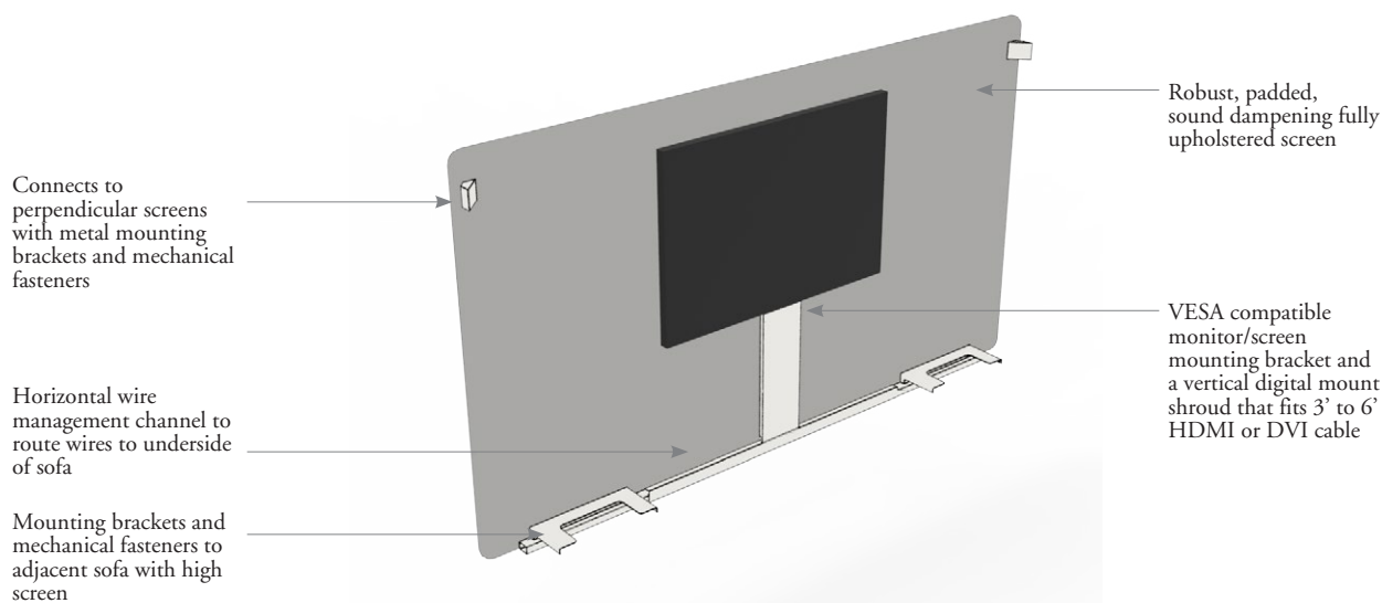
Banqs High Spanning Screen, 84" Digital Share & Worksurface Electrics (NBAZD Shown)
