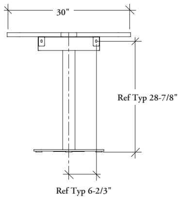
Banqs table with flat base, 30d x 72w, Zones Small Power Pill
