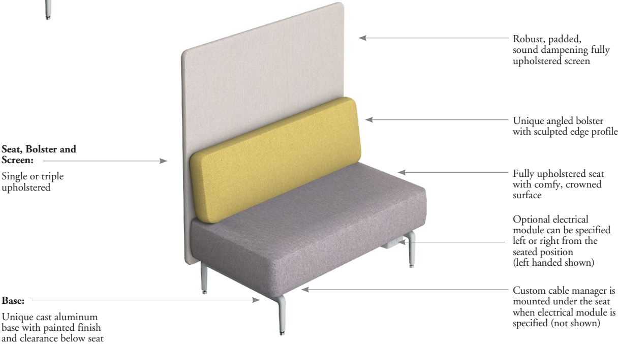
Banqs – Single-Sided Sofa, High Back
