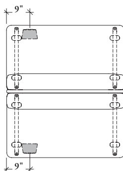
48" wide single-sided sofa and electric module (Mixed Right and Left from seated position shown)
