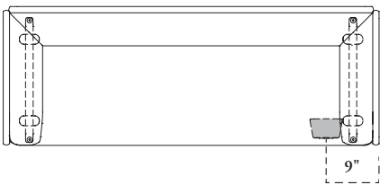
72" wide Full Alcove Sofa and electric module
