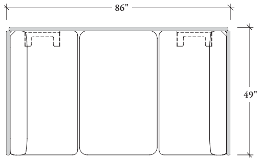
Single-Sided Sofa, High Screen, 2-Seat with 30" deep x 48" wide Table
