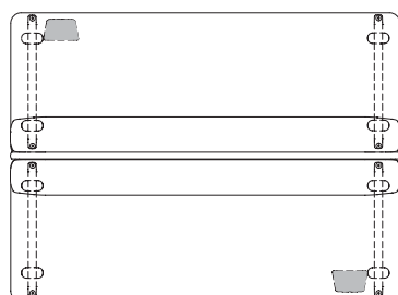
72" wide back-to-back sofa and electric module (left from seated position shown)
