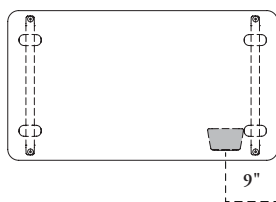
48" wide bench with no back and electric module (left from seated position shown)
