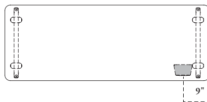
72" wide bench with no back and electric module (left from seated position shown)
