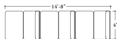
Open Planning with Banqs Back-to-Back Sofas, High Screens and Banqs Single-Sided Sofas, High Screens
