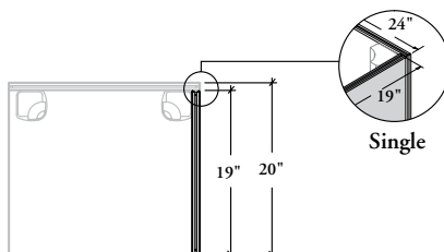
Recessed Size – Lateral
