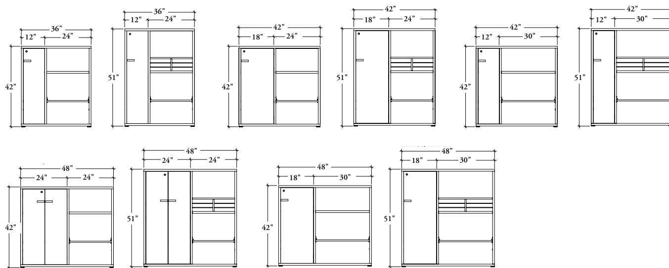
Extended Supporting Tower with Full Door (RBXTS or RBXTW)
