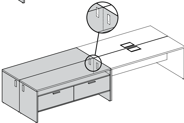
Wire Management Clips (underneath worksurface)
