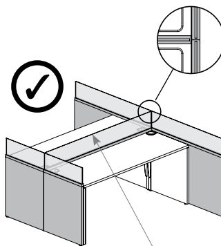
With Add-On Screen or Central Screen
