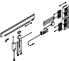
M F T W E P F Tek Work Electrical Power Kit for Fixed or No Worksurface Plug-In
