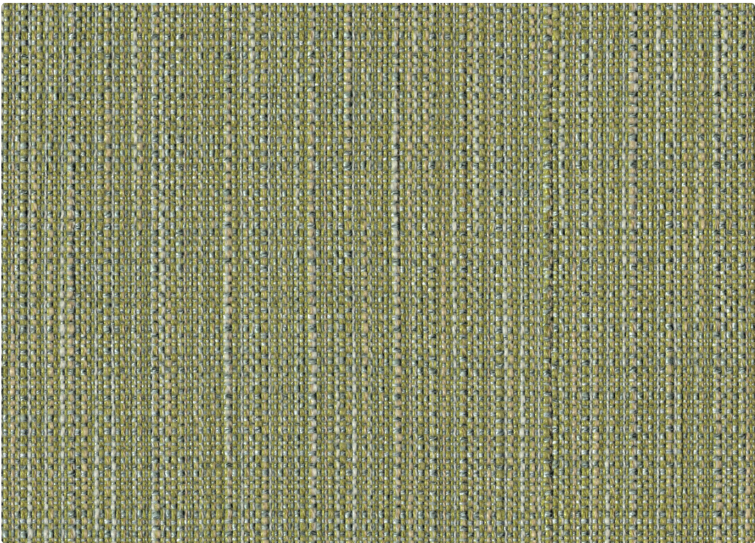
Isotope 4109-12
