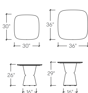
Ora Square Work Table (TKQ2C or TKQ2E base / TKQ1S top)
