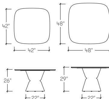
Ora Square Work Table (TKQ2D or TKQ2F base / TKQ1S top)
