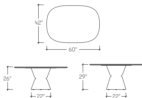
Ora Rectangle Work Table (TKQ2D or TKQ2F base / TKQ1T top)
