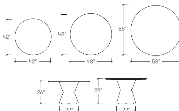
Ora Round Work Table (TKQ2D or TKQ2F base / TKQ1R top)
